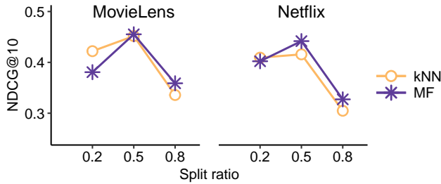
Fig. 2: System scores: NDCG@10 for kNN and MF varying (only) the test/train split ratio (A2). All other settings are as specified for the starting point. Similar behavior arises with Prec@10. The p values for a paired two-tailed t -test are essentially 0 for all the comparisons, except in MovieLens at a 0.5 split ratio where the p value is 0.897.
